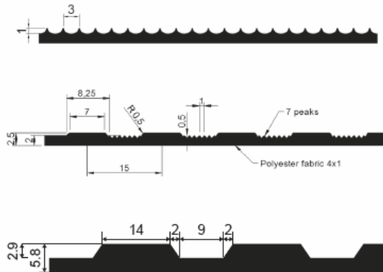
Rectangular ribbed (MR)
